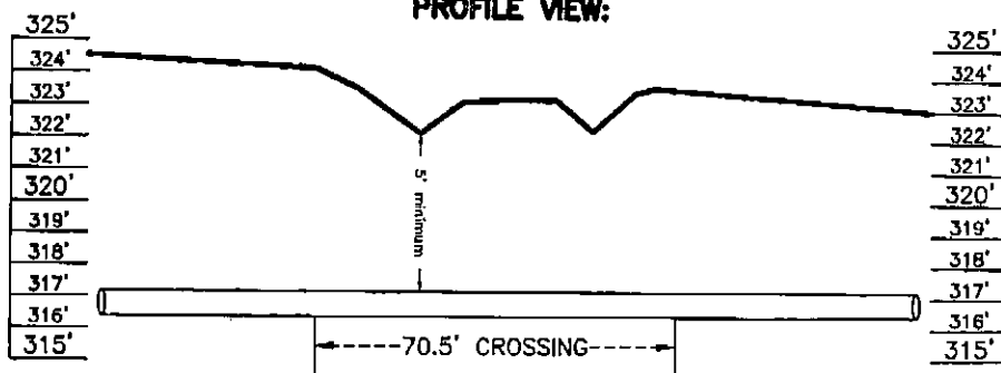
PROFILE VIEW:
